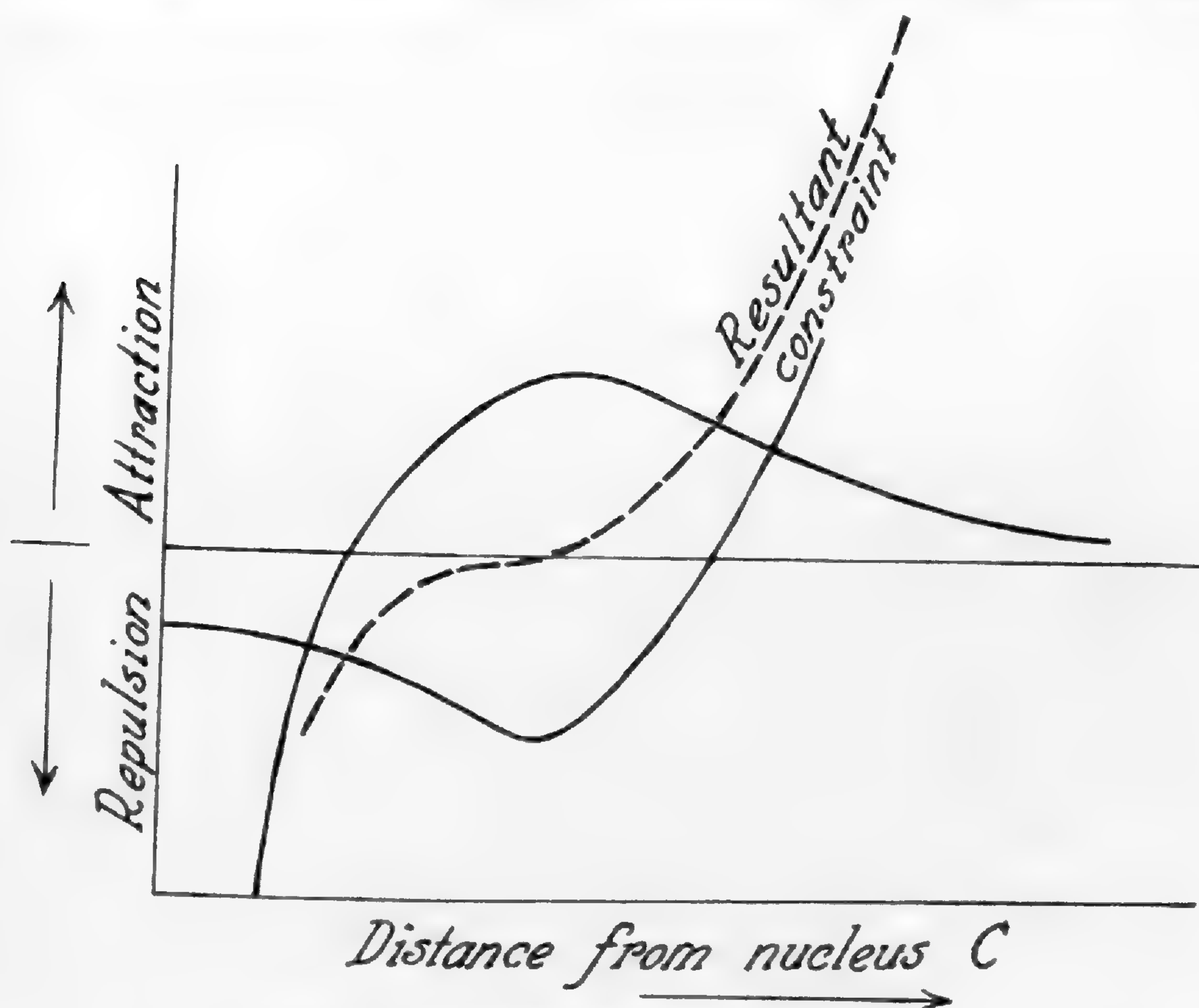
FIG. 3. Symmetrically weak union; loose electron.
